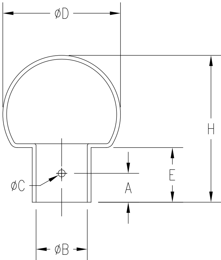
SLIP-ON
